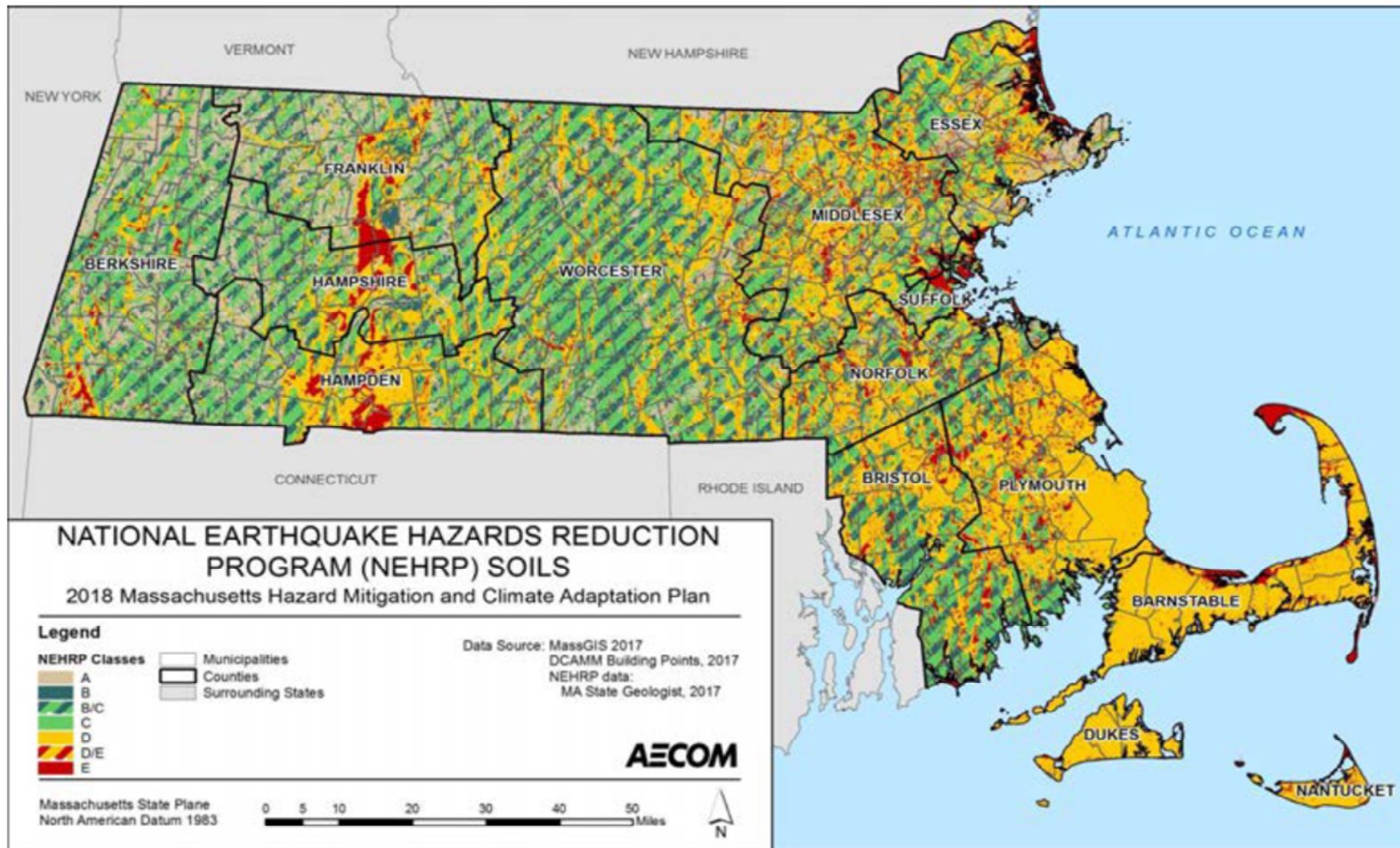
Figure 3-14: National Earthquake Hazards Reduction Program Soil Types in Massachusetts
