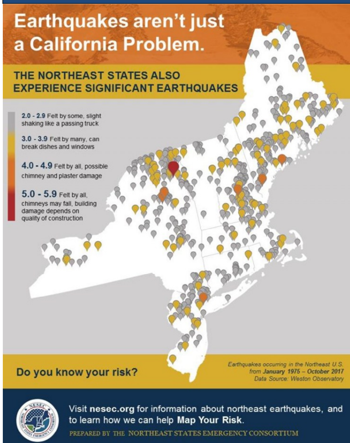
Figure 3-15: Earthquakes Occurring in the Northeast from 1975 - 2017
