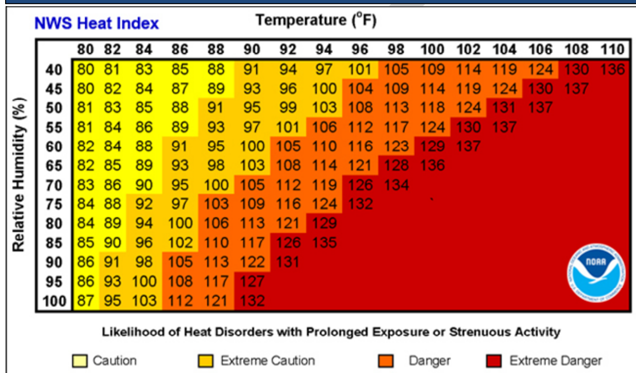
Figure 3-24: National Weather Service Heat Index
