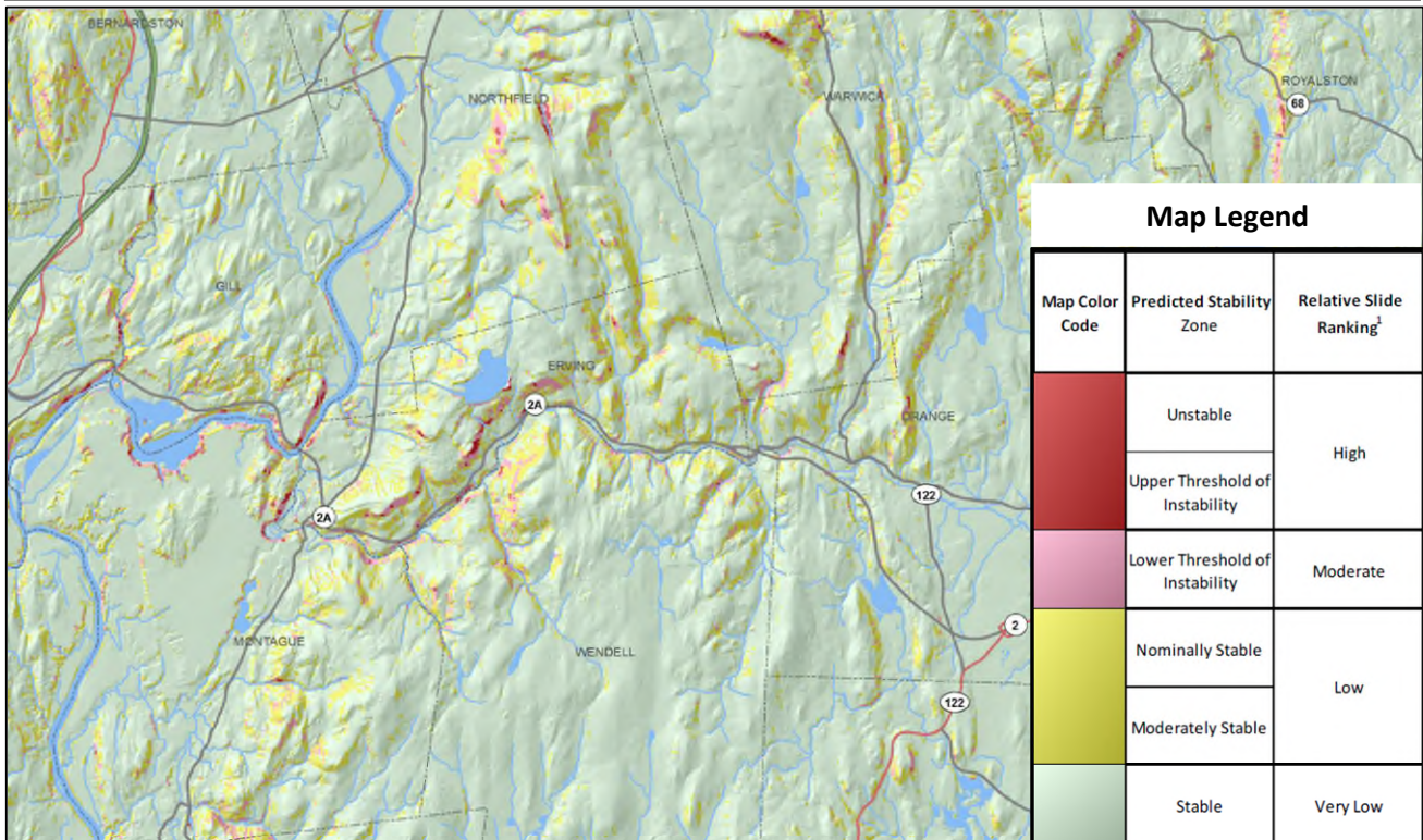
Figure 3-20: Slope Stability Map, Erving and Surrounding Towns
